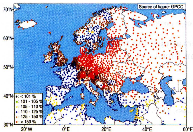
Fig. 2. Monthly mean of correction for systematic measuring errors in % of measured precipitation totals using Legates' (1989) monthly correction factors on a 0.5°-grid. Analysis month: January 1999.
