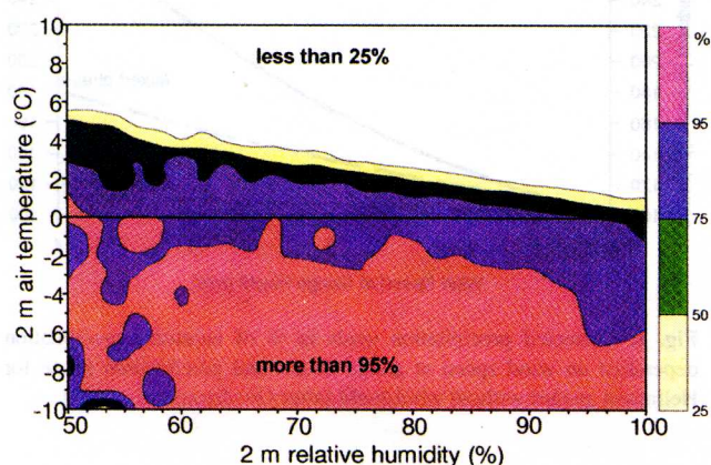
Fig. 4. Percentage of probable occurrence of solid precipitation in daily precipitation totals dependent on 2 m air temperature and 2 m relative humidity. Derived by GPCC from more than 600 000 GTS-SYNOP reports of 16 winter months 1995-1999.
