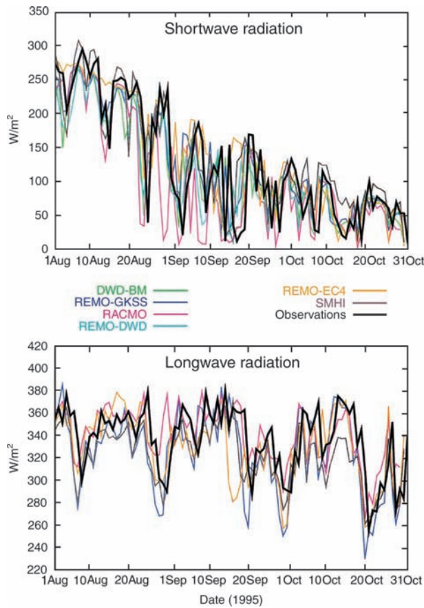
Fig. 6. Downwelling short-wave (upper panel) and long-wave (lower panel) surface radiation fluxes ( \text{W/m}^2 ) at Lund in southern Sweden
