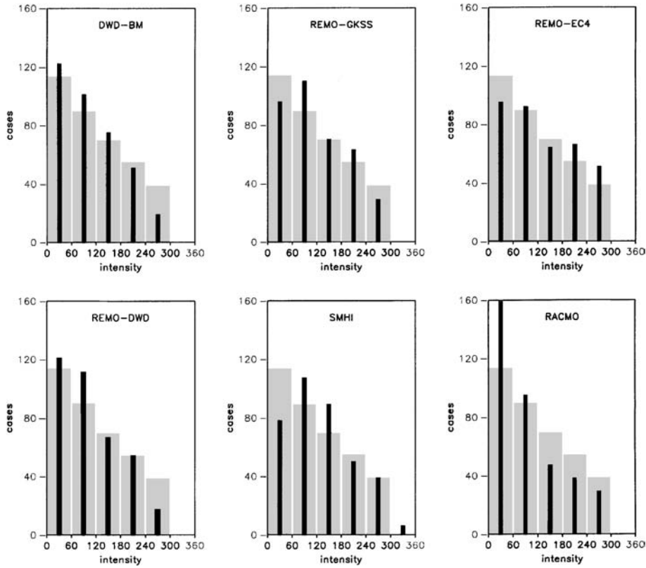
Fig. 7. Histograms of observed and modelled daily mean downwelling short-wave fluxes ( \text{W}/\text{m}^2 ) at the surface during August, September and October 1995, for ensembles of the stations Schleswig, Lund, Borlänge and Luleå. The observed distribution is shown by shaded rectangles and the model results by black columns
