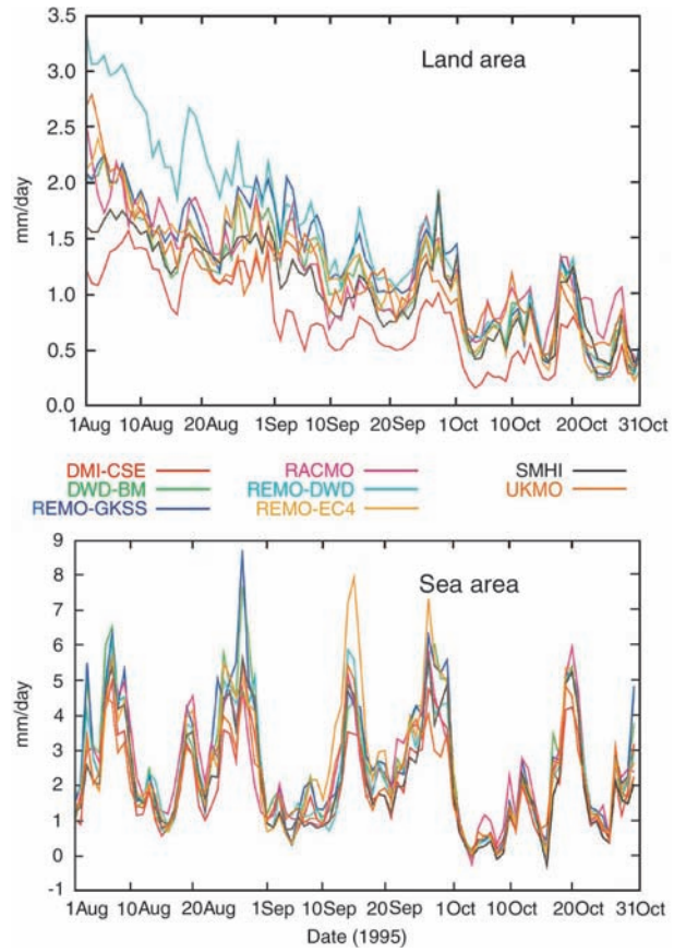
Fig. 11. Daily means of evaporation (mm/day) from the land surface (upper panel) and sea and lakes (lower panel) inside the Baltic Sea catchment area
