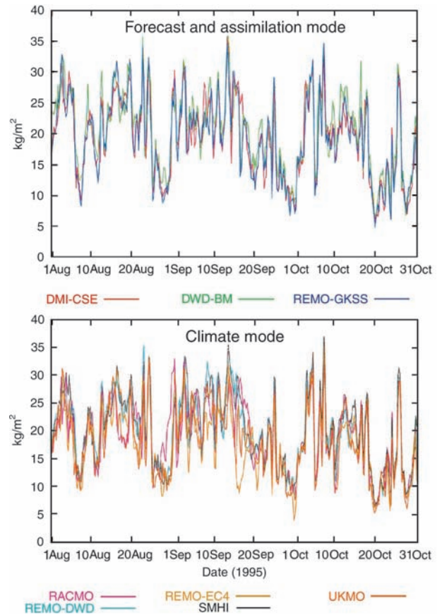
Fig. 3. Time series of the mean 6 h vertically integrated specific humidity ( \text{kg/m}^2 ) at the station Haessleholm (Sweden) from GPS observations and models in assimilation and forecast mode (upper panel) and observations and models in climate model (lower panel)
