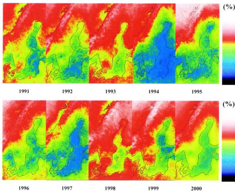
FIG. 9. Summer cloud frequencies (%) over Scandinavia in the period 1991–2000 derived from NOAA AVHRR data.
