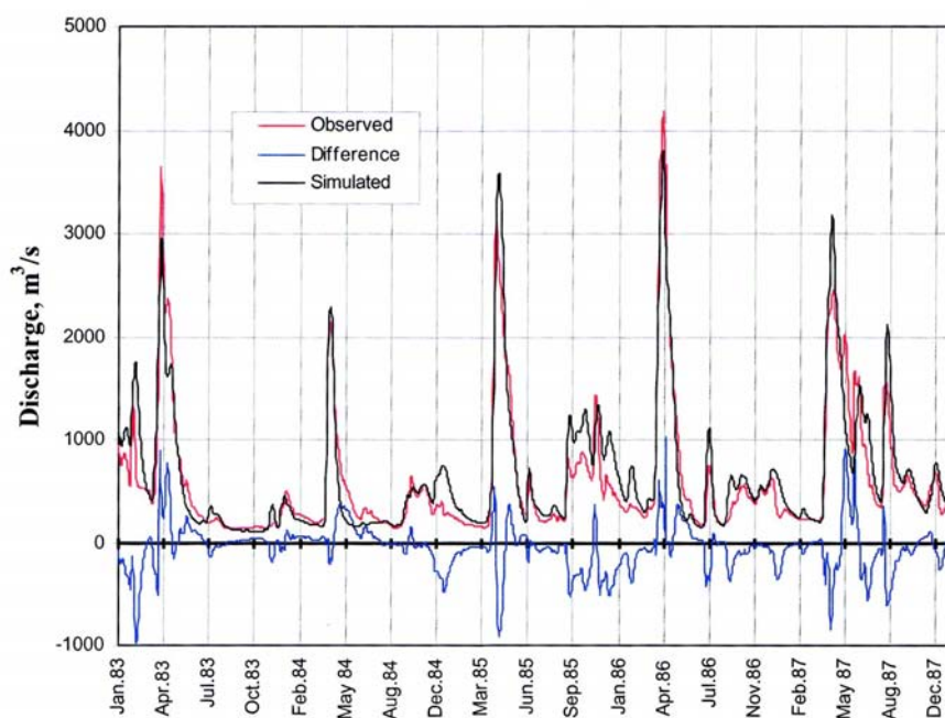
FIG. 14. Runoff of the Daugava measured at station Plavinas (Latvia) and simulated for the same position with the METQ98 model on the basis of meteorological input data.
