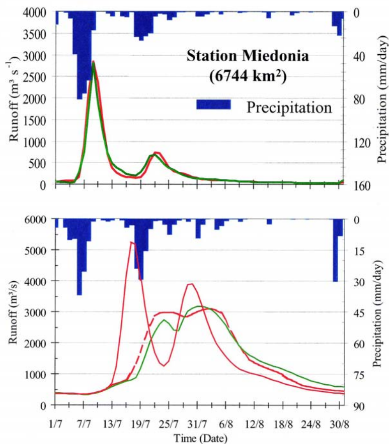
FIG. 18. Measured and modeled hydrograph at stations Miedonia (upper panel) and Gozdowice (lower panel) during the Odra flood in July 1997.
